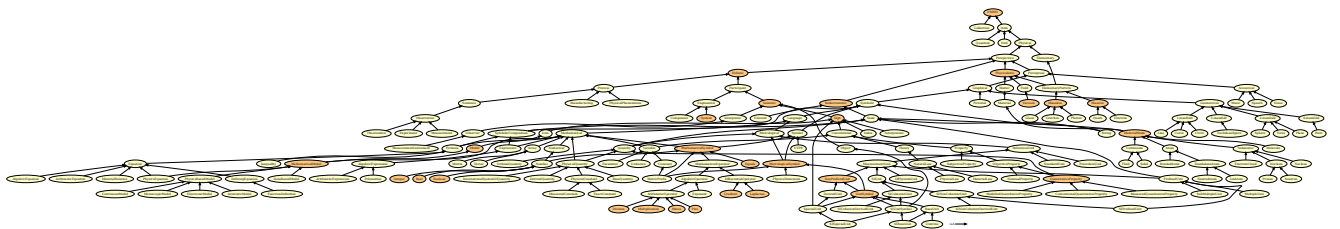
Figure 5.2: The almost complete taxonomy of EMMO classes. Only physical quantities and constants are left out.
